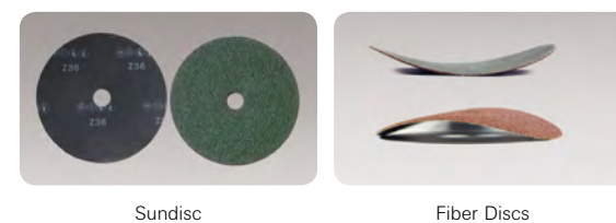
Warping comparison test in humid conditions between Sundisc and Fiber Discs. (77 F, Humidity 45% - after 24 hours)
